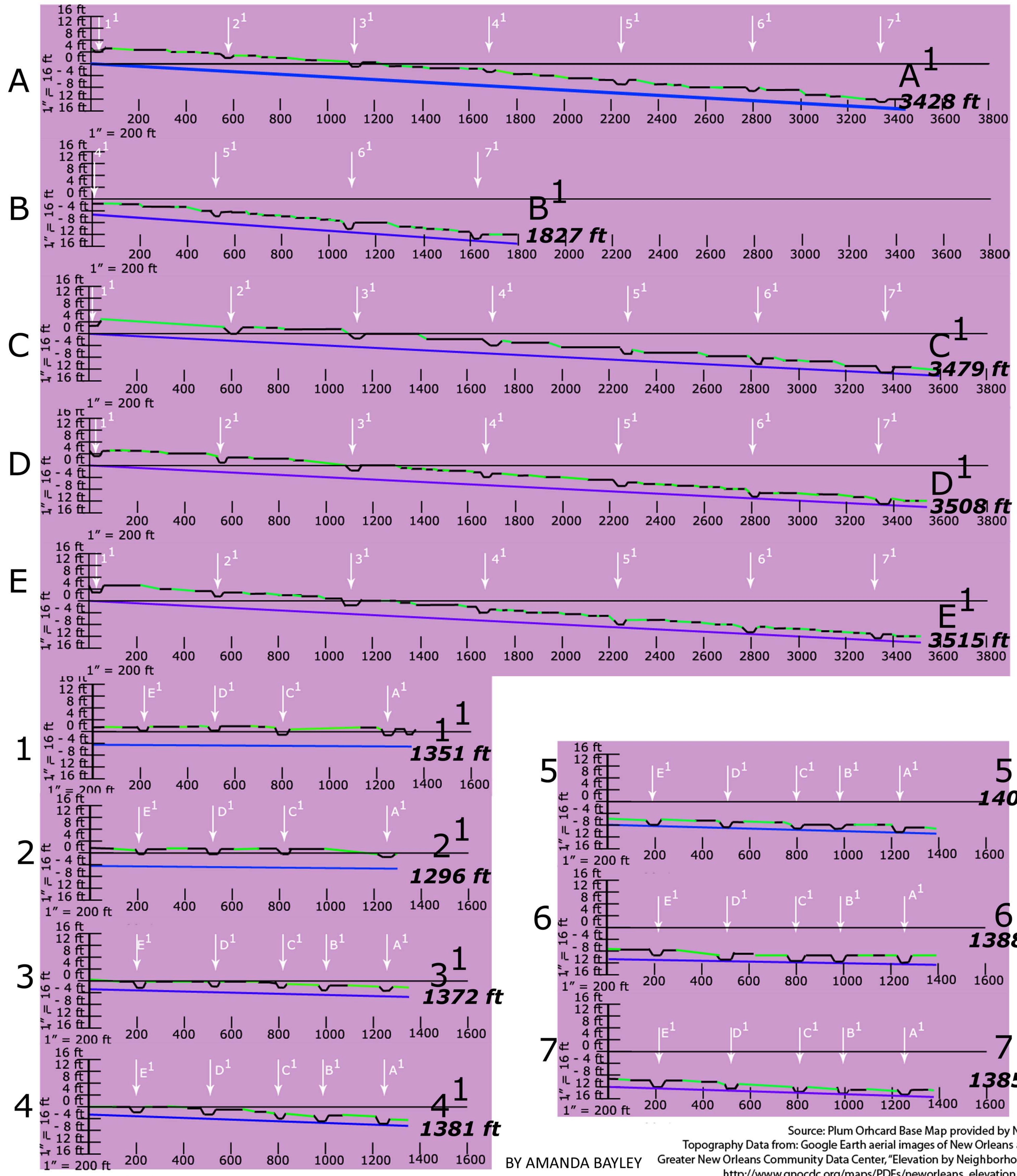
PLUM ORCHARD: Cross- Sections by Street
